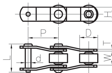
Type B Chain
