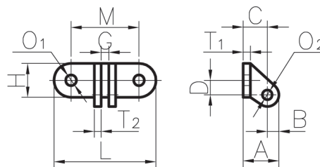
Dimension Diagram of Flight Wing Attachment (C Type)
