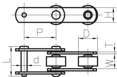
Type A Chain
